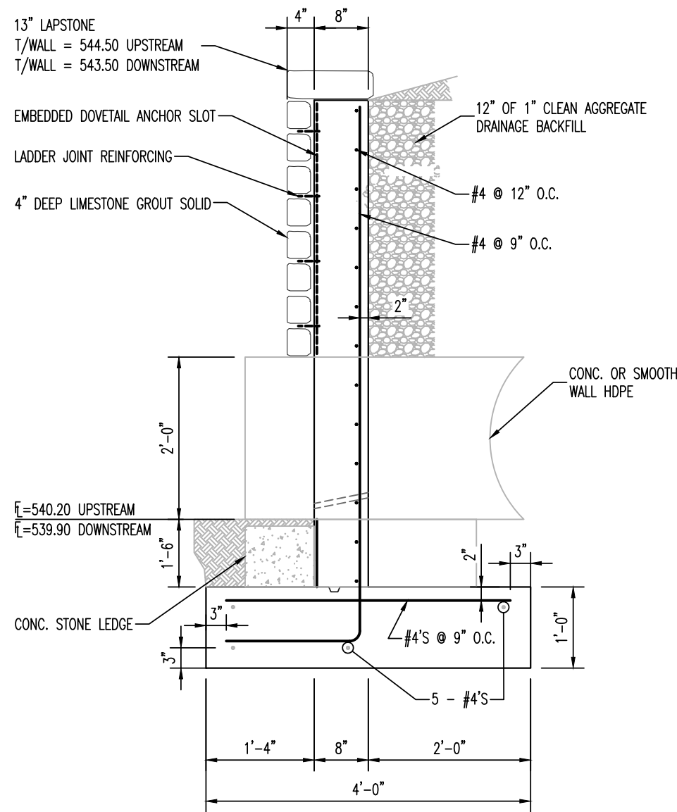
CANTLEVERED RETAINING WALL @ STATION 83+76 SCALE: N.T.S.
