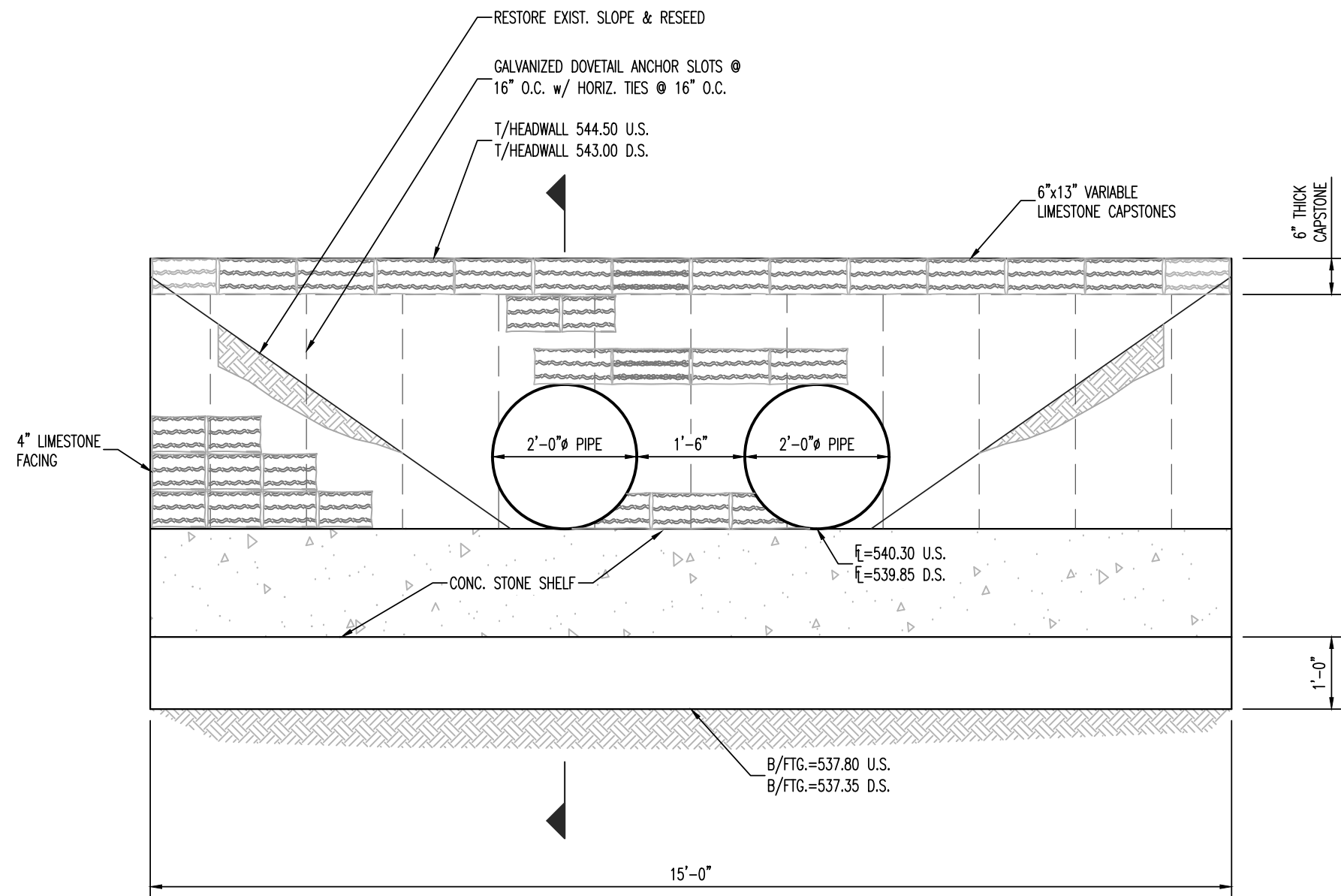
HEADWALL ELEVATIONS @ STATION 83+76 SCALE: 1/2" = 1'-0"
