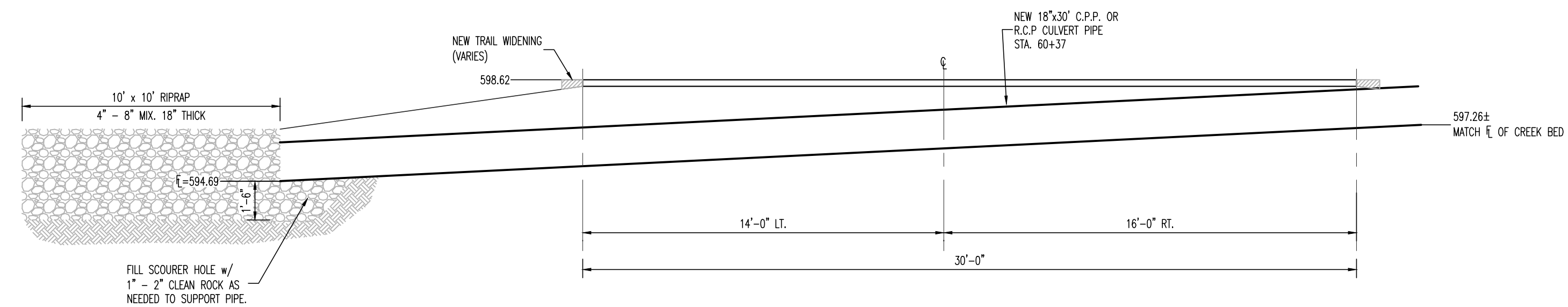
PROFILE @ STATION 60+37
