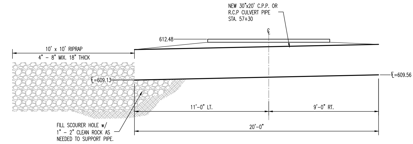
PROFILE @ STATION 57+29
