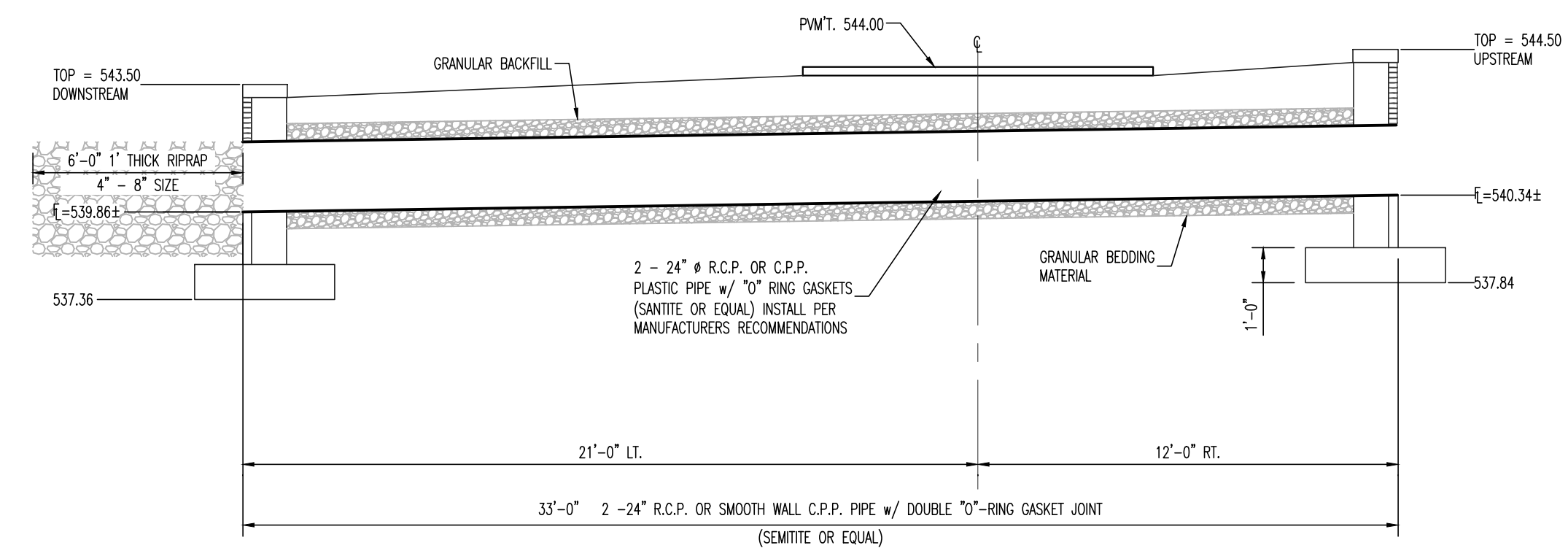
PROFILE @ STATION 83+76
