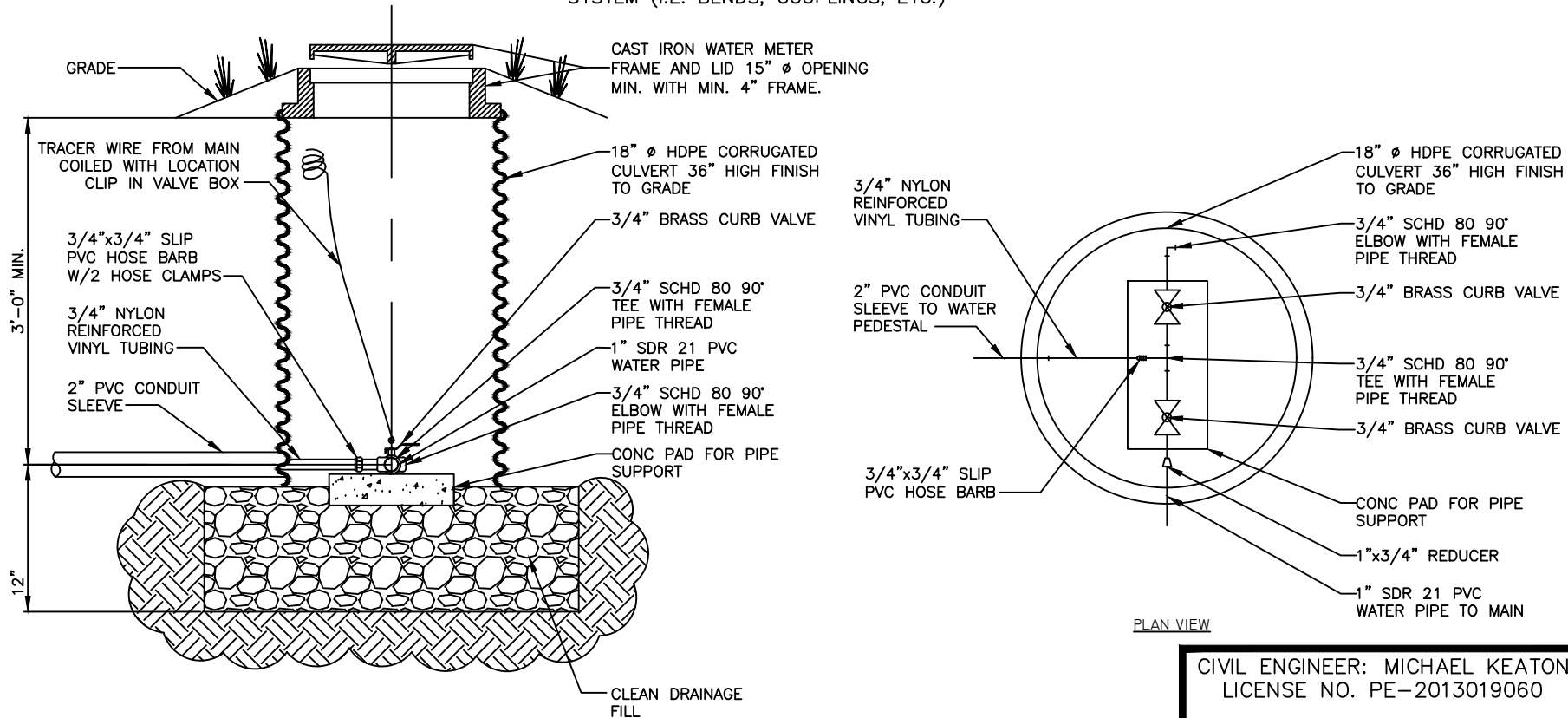
3 VALVE BOX - CAMPSITE C-503 NTS
