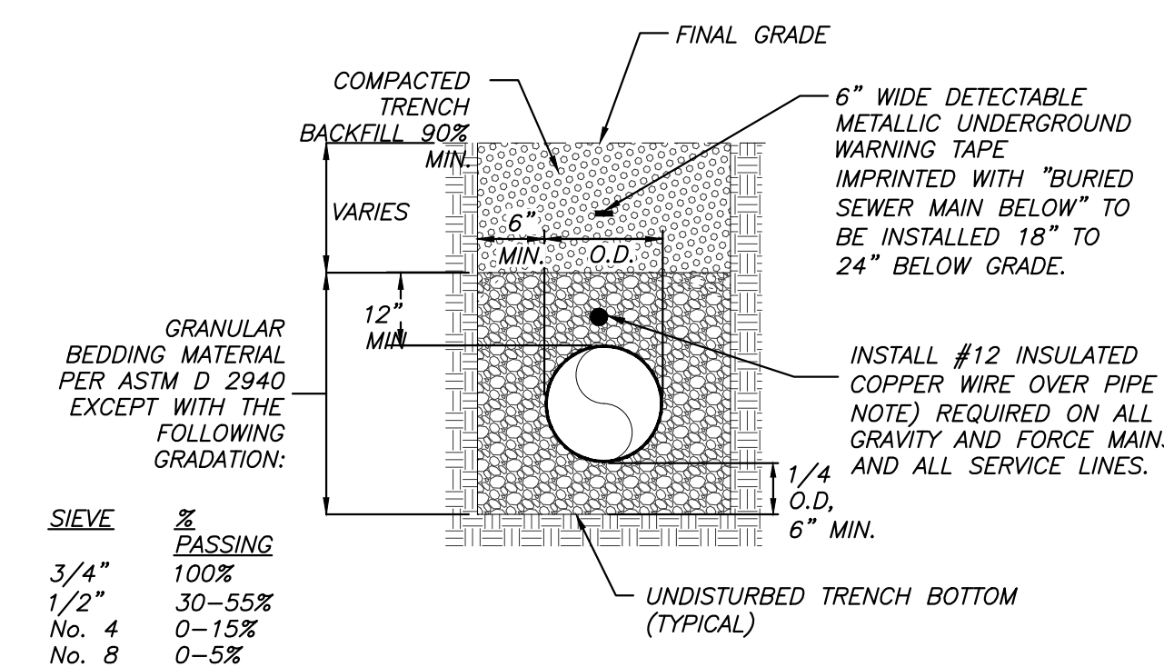
SINGLE PIPE IN TRENCH PIPE INSTALLATION DETAIL NOT TO SCALE
