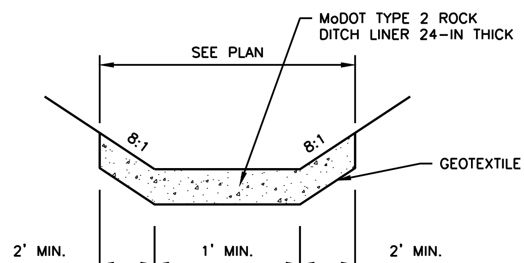
I ROCK OUTLET SECTION NOT TO SCALE
