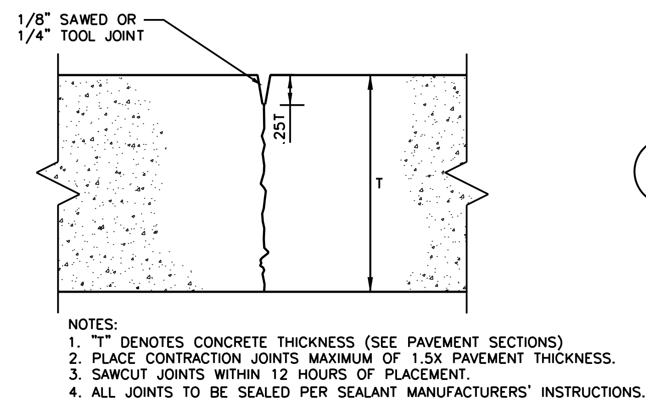
F CONTRACTION JOINT NOT TO SCALE
