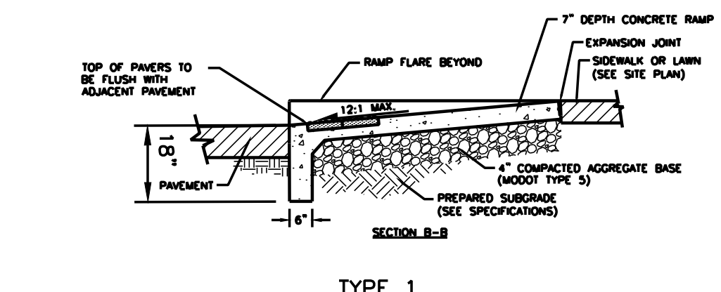
J SIDEWALK RAMP NOT TO SCALE
