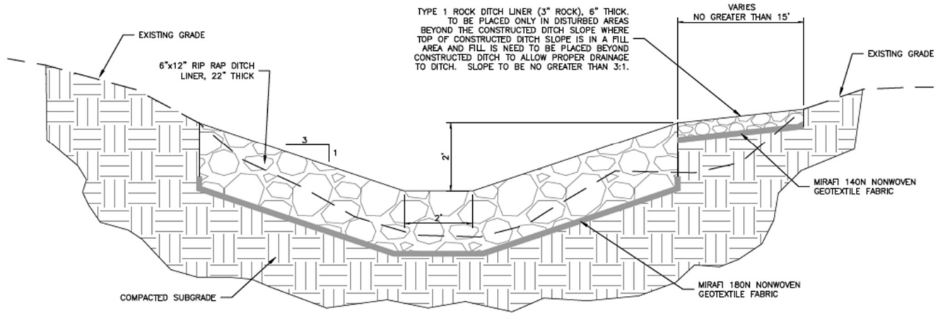
TYPICAL RIP RAP CHANNEL DETAIL NO SCALE
