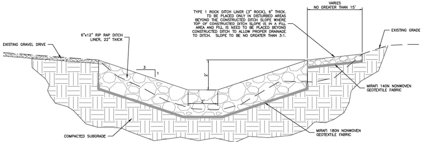
TYPICAL RIP RAP CHANNEL ALONG GRAVEL DRIVE DETAIL NO SCALE
