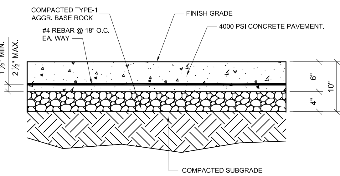
2 TYP. CONCRETE PAVEMENT C-101 SCALE: 1\"/>
