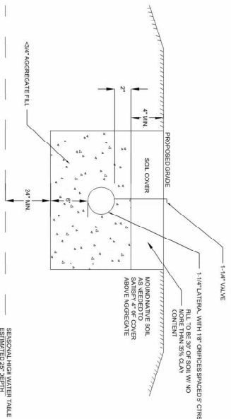
3 TYPICAL TRENCH C101 SCALE: NTS
