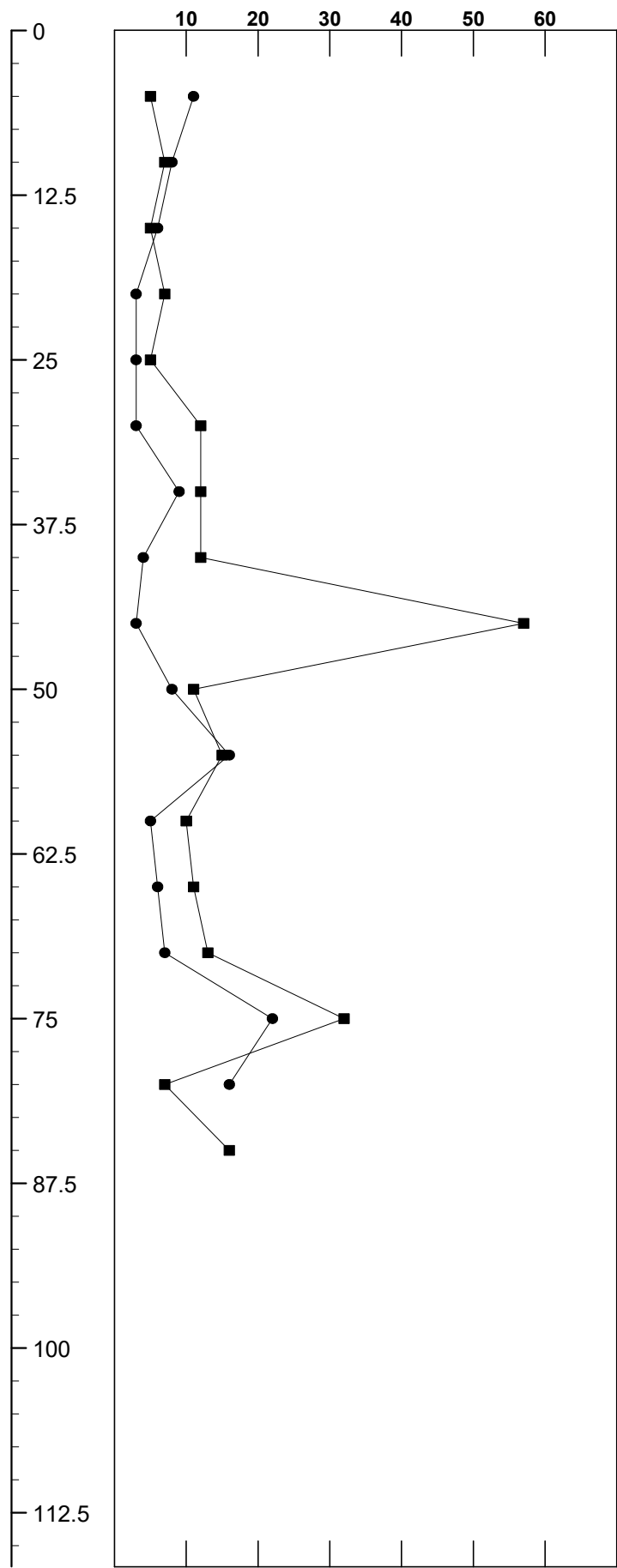
SPT N-VALUE
